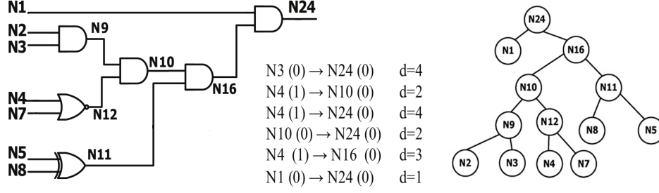
Figure 1: Example circuit with implications and graph representation, from [8]
